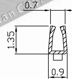
SEC C-C
